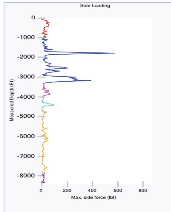
Figure 2 - Side Loading of Well in Reducing Rod Parts Case Study.
